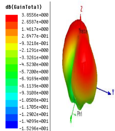
Fig.12: Gain at 3.17GHZ
