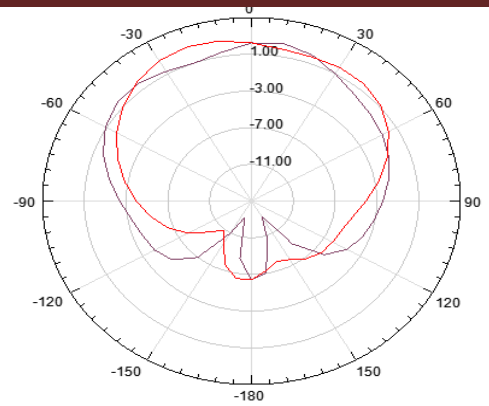
Fig.11: Radiation pattern at 3.17GHZ
