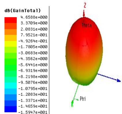
Fig.6: Gain at 1.57GHZ
