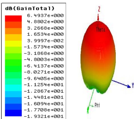
Fig.8: Gain at 1.95GHZ
