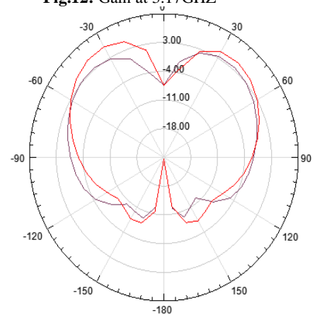
Fig.13: Radiation pattern at 4.05GHZ
