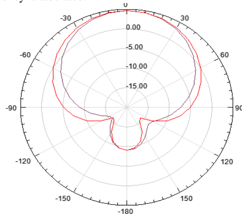
Fig.5: Radiation pattern at 1.57GHZ
