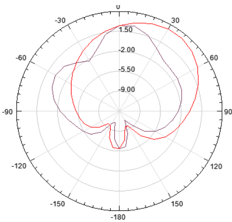
Fig.9: Radiation pattern at 3.11GHZ
