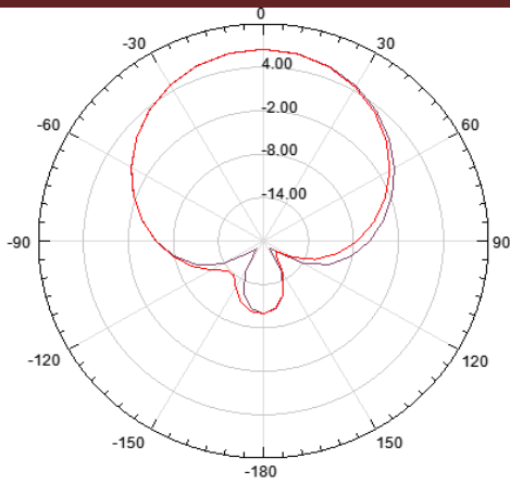
Fig.7: Radiation pattern at 1.95GHZ
