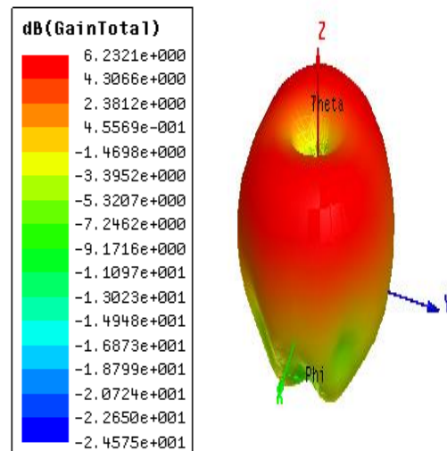
Fig.14: Gain at 4.05GHZ
