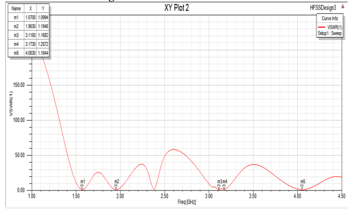
Fig.4: VSWR
