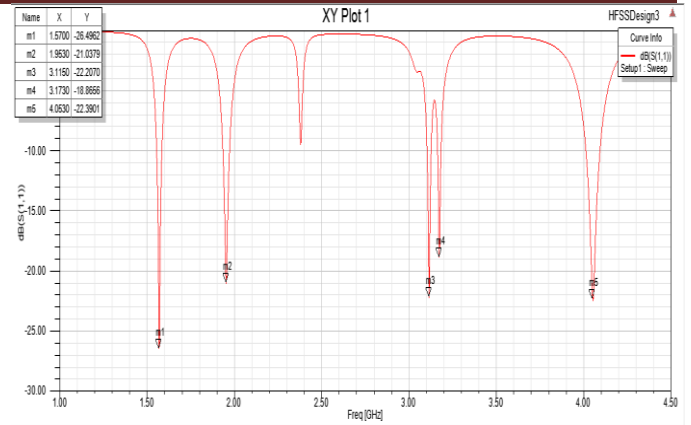
Fig.3: Return loss
